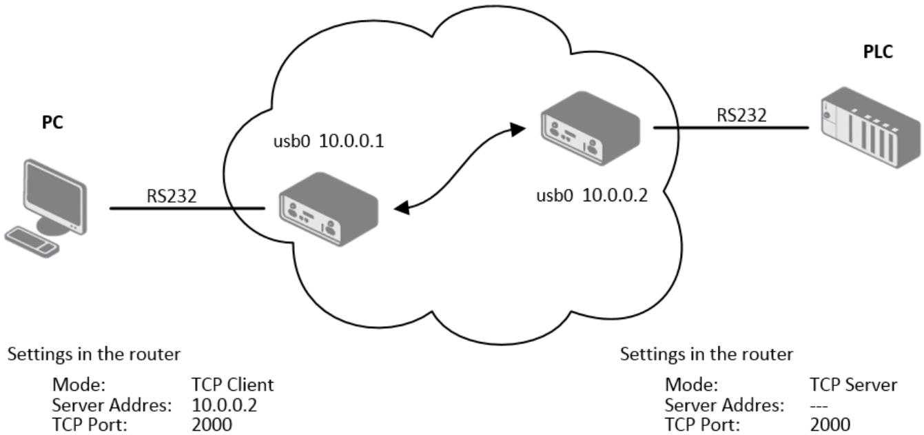
Figure 86: Serial interface configuration example
