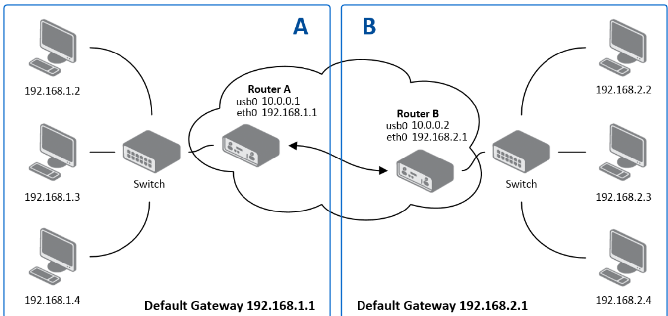
Figure 68: An example of L2TP topology
