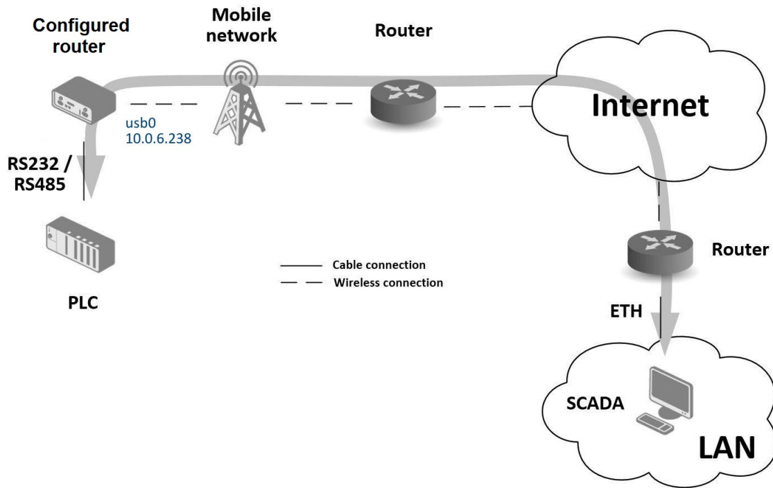
Figure 128: Serial Gateway – sample topology
