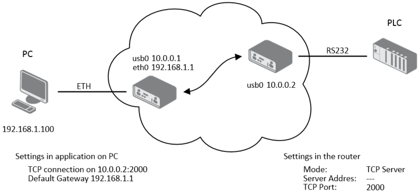
Figure 85: Ethernet-to-serial communication configuration example
