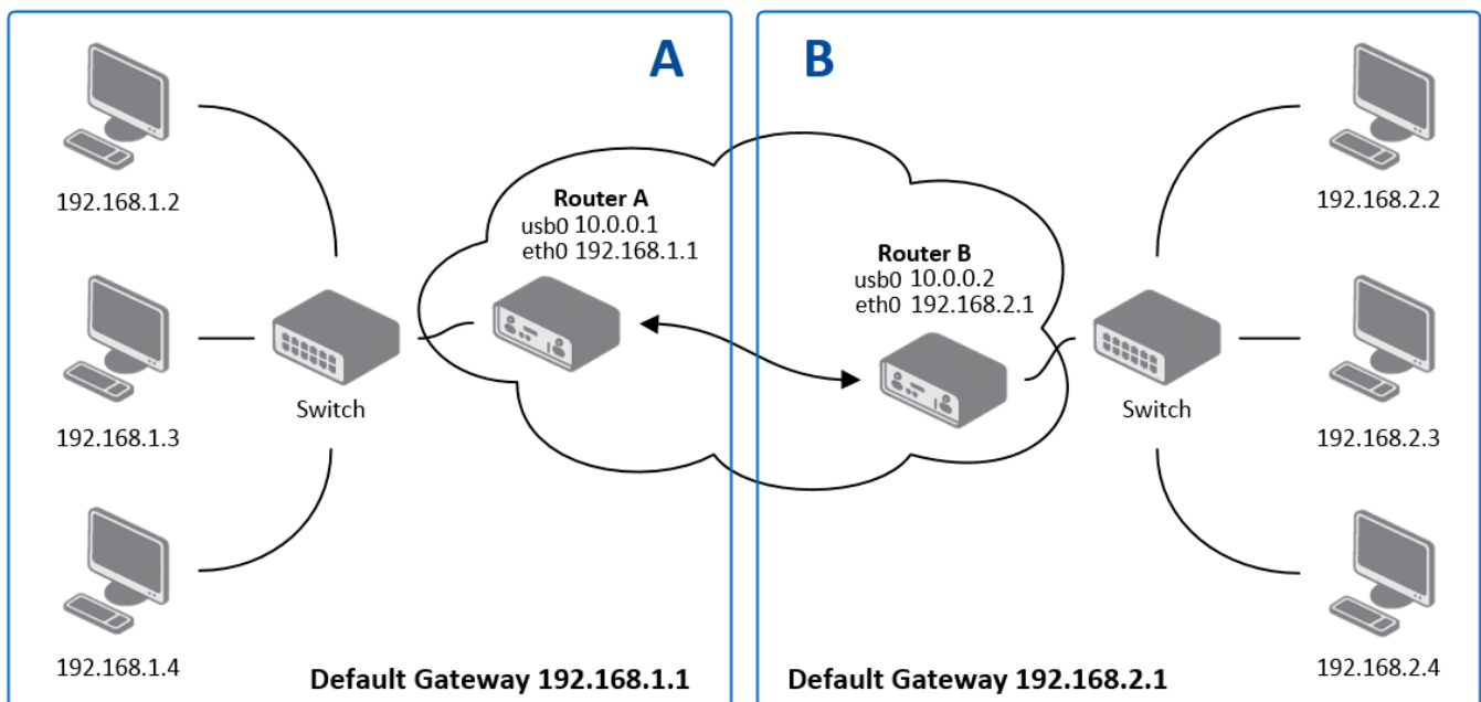
Figure 70: An example of PPTP topology
