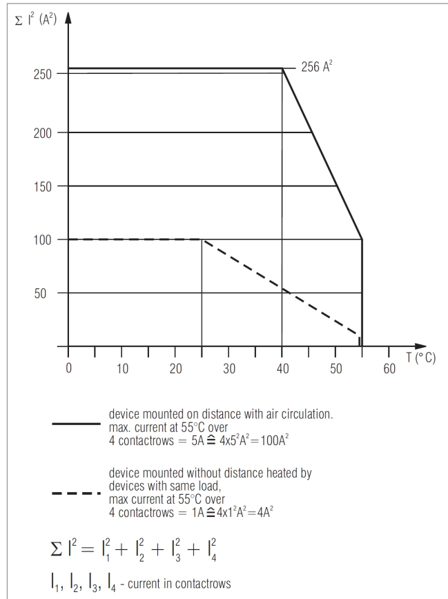
Total current limit curve
