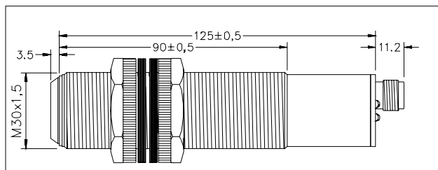
Dimensions/Abmessungen/Dimensions
