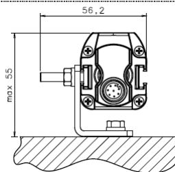
MOUNTING B
