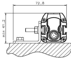
MOUNTING A
