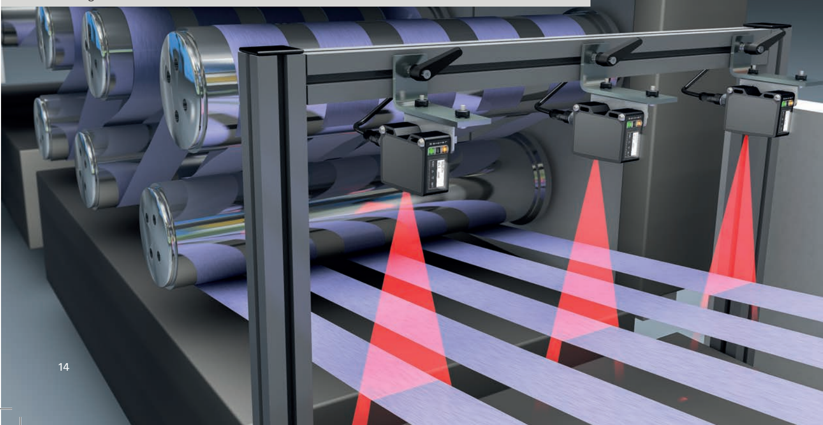
The light section sensors were installed above the bitumen sheet that has to be monitored.
