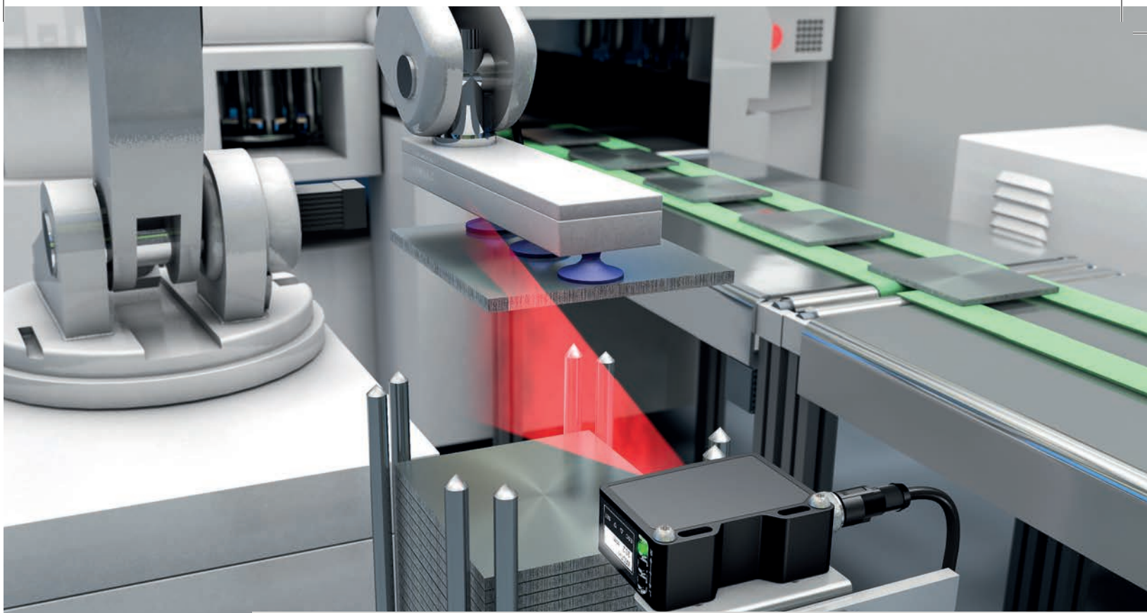
The light section sensor was installed in such a way that it could laterally detect the lifted metal blank.
